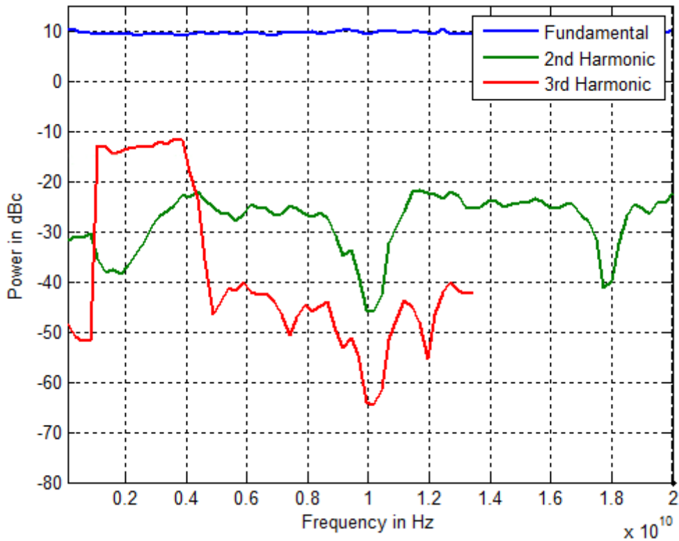
Harmonics @ 10 dBm
