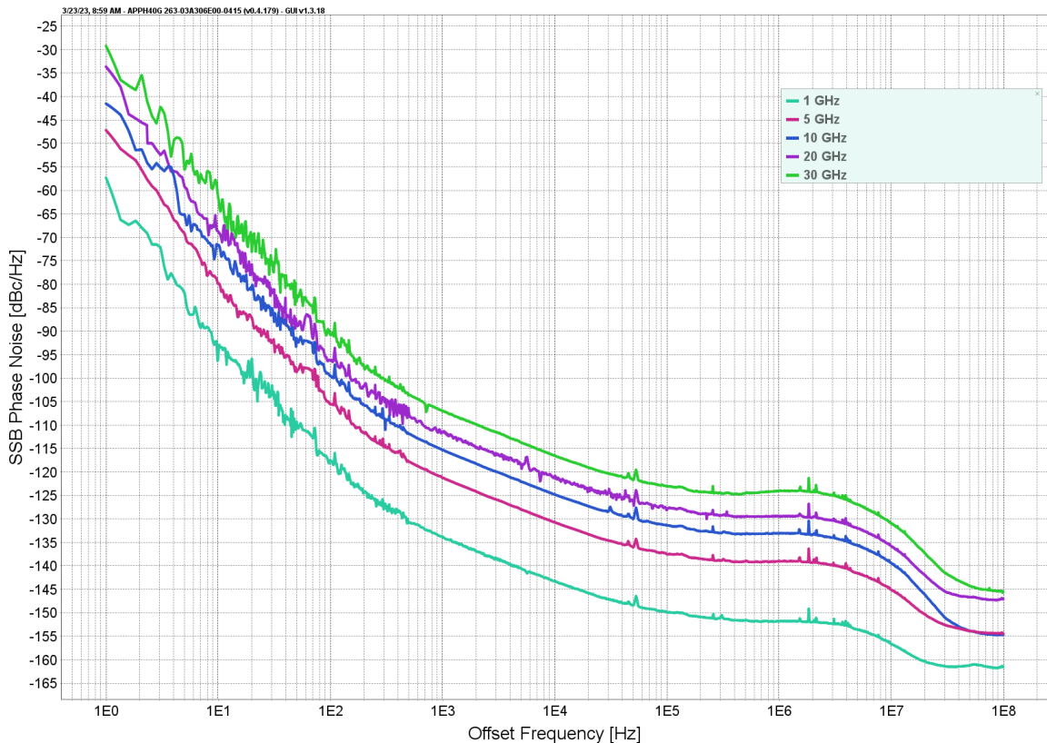
SSB Phase Noise Performance
