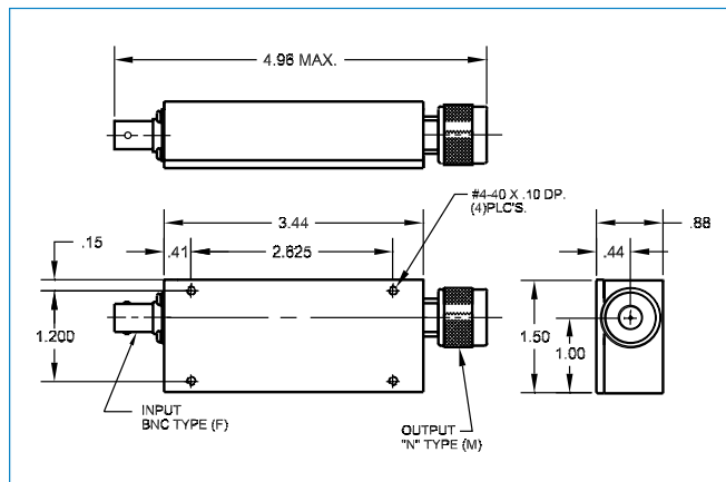
NC3405, 06, 07 Dimensions (inches)
