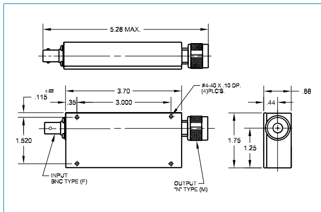
NC3404 Series Dimensions (inches)
