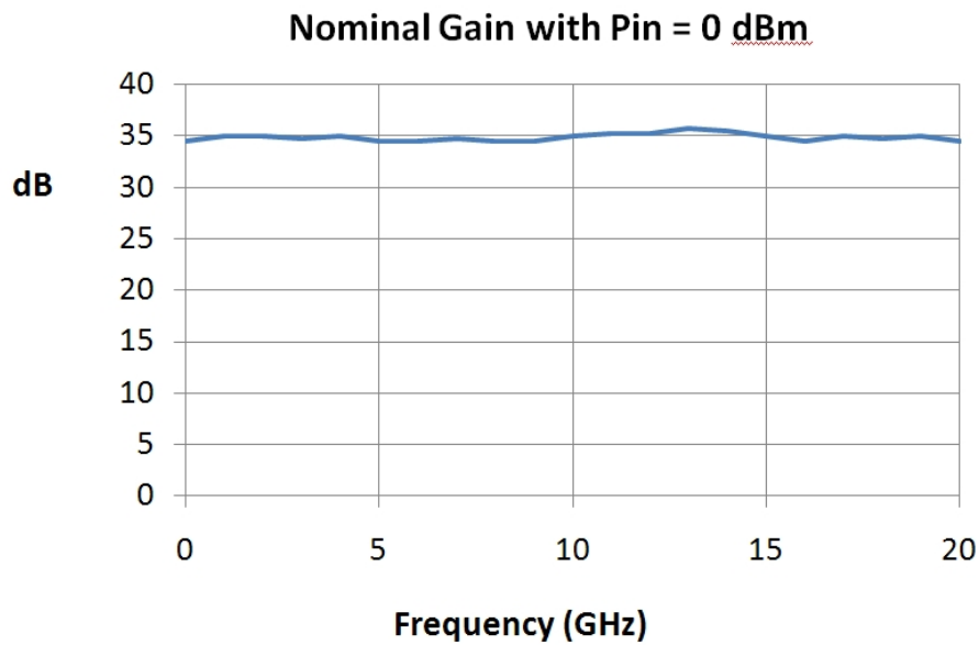
Figure 4: Gain (nominal)
