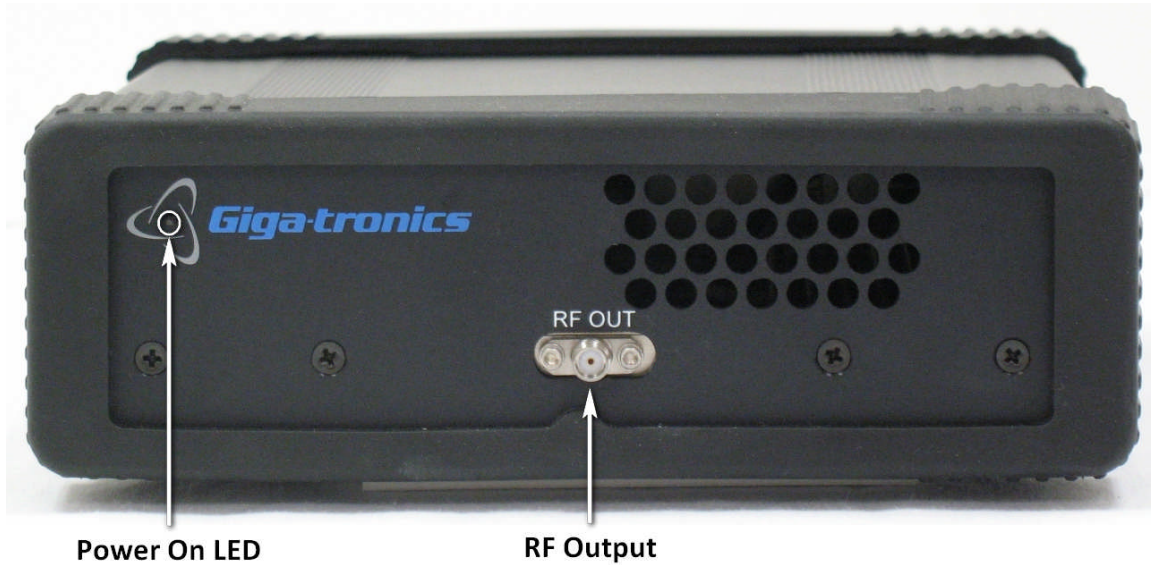
Figure 1: GT-1020A Front Panel
