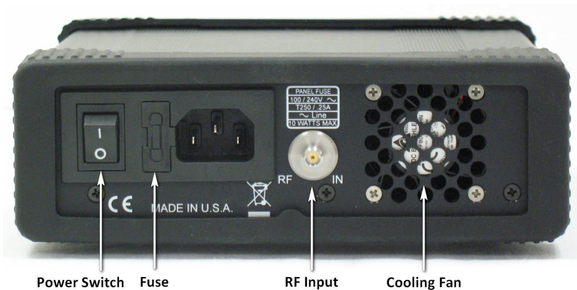
Figure 2: GT-1020A Rear Panel
