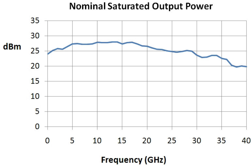
Figure 3: Saturated Output Power (nominal)
