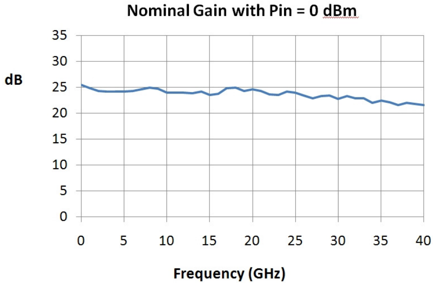
Figure 4: Gain (nominal)
